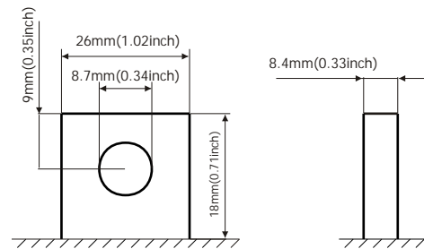
Terminal Dimensions
