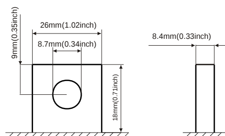
Terminal Dimensions
