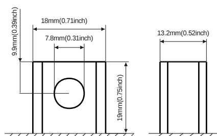
Terminal Dimensions
