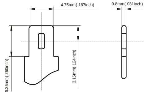
Terminal Dimensions
