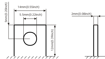
Terminal Dimensions
