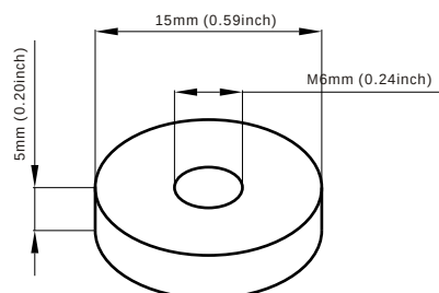
Terminal Dimensions
