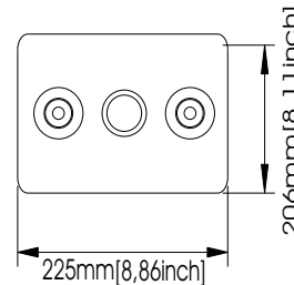
Terminal Dimensions
