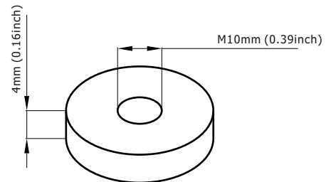
Terminal Dimensions
